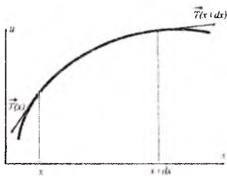
III.1-rasm: Torning ko'ndalanga tebranishiga doir
