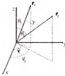
1.3-rasm: Qo'shish teoremasiga oid
