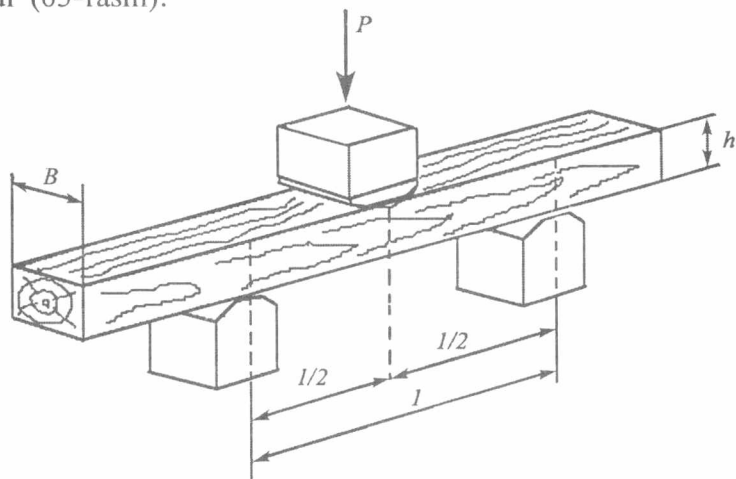
65-rasm. Yog'ochni tashqi kuchga ta'sirini kuzatish.
