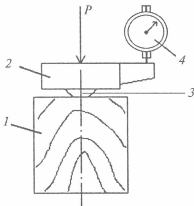
67-rasm. Yog'och tanasining statik qattiqligini sinash shakli:
