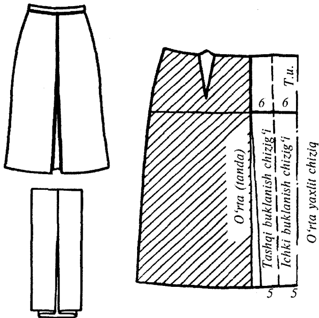
3.7-rasm. Taxlamalarni qurish.
