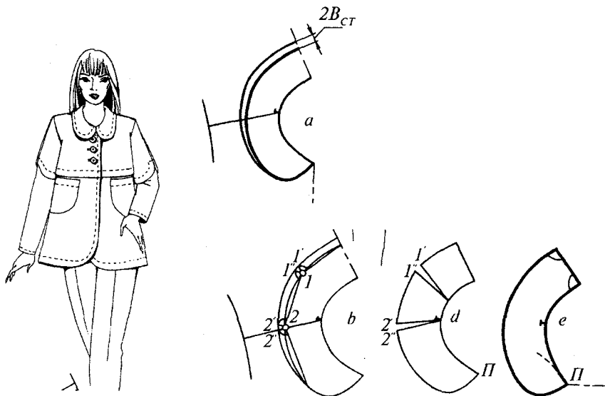
3.14-rasm. Yassi yoqa:
