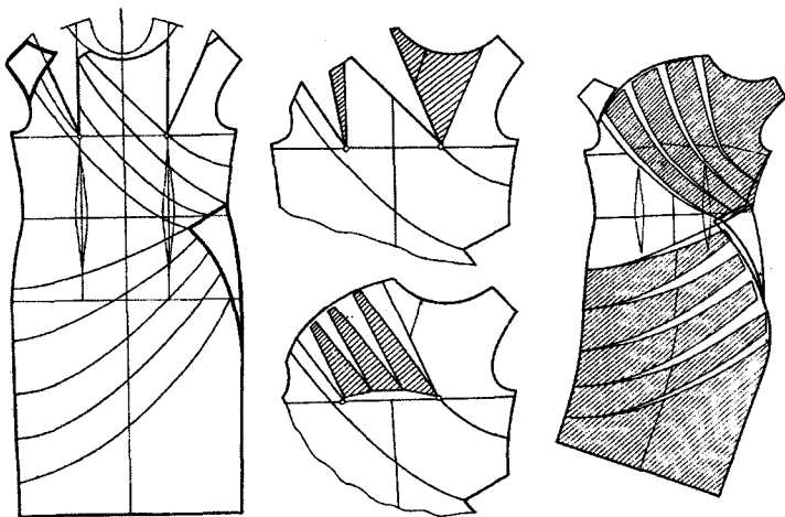
3.13, a, b-rasm. Yumshoq taxlama va qirqmalarning chizig'ini qurish.
