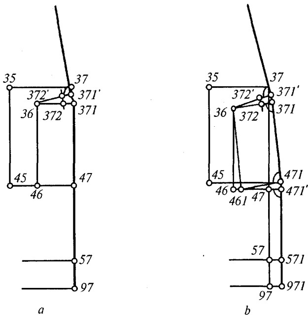
2.18-rasm. Kiyimning old o'tar chizig'ini qurish:
