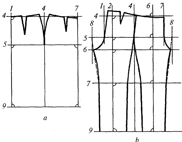
2.3-rasm. Tananing pastki qismiga mos kiyim bazis to‘rining chiziqlari: a — yubkaga oid; b — shimga oid.
