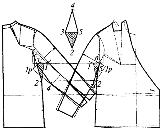
3.30-rasm. Tipaviy konstruksiya asosida yaxlit bichilgan yengni qurish: a — yumshoq shaklli bichim; b — xishtakli bichim.
