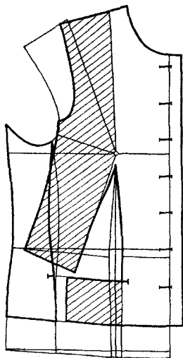
3.4-rasm. Cho‘ntak chizig‘iga o‘tadigan bel vitachkasiga ko‘krak vitachkasini o‘tkazish.
