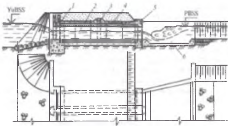
5.15-rasm. Quvurli inshoot: 1 kirish kallagi; 2–quvur; 3 filratsiyaga qarshi diafragma; 4 loyli grunt; 5 chiqish kallagi; 6- suv qudug‘i.
