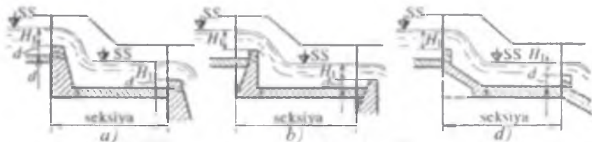
5.28-rasm. Sharshara tushish devorlari:
