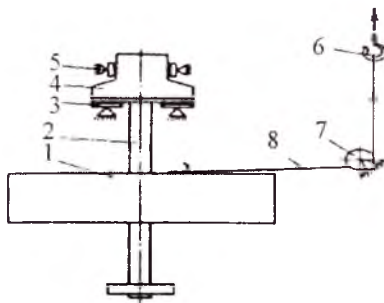
4.14-rasm. Gidroagregatning generator rotorini spitsalari ortiga burish:
