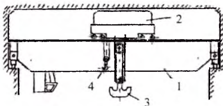
1.12-rasm. Kc'priksimon kran sxemasi
