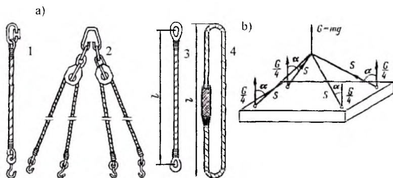
4.6-rasm. Takelaj jihozi uchun stropillar
