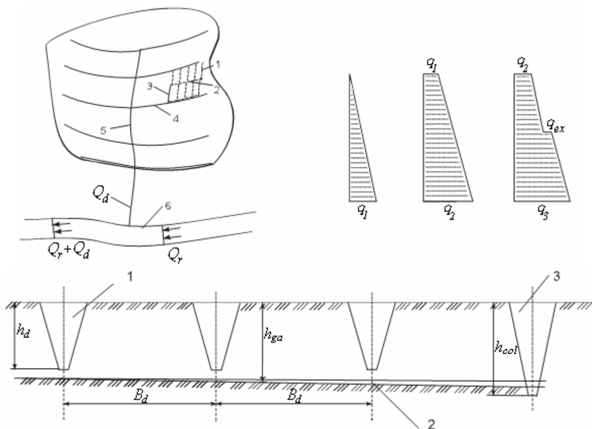
118-rasm. Zax qochirish tizimi sxemasi:
