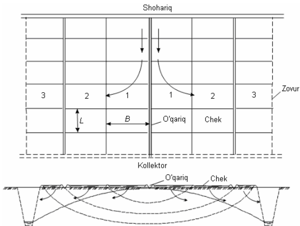
93-rasm. Sho‘r yuvish jarayoni sxemasi
