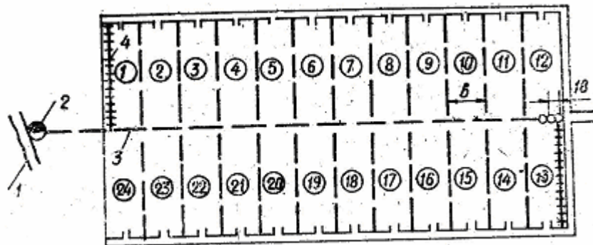
84-rasm. "Voljanka" rusumli yomg'irilatib sug'orish mashinasi yordamida sug'oriladigan madaniy yaylov sxemasi:
