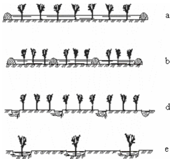
7-rasm. Yer ustidan sug‘orish usulining tasnifi:
