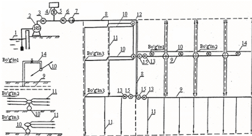
33-rasm. Tomchilatib sug'orish tizimi sxemasi:
