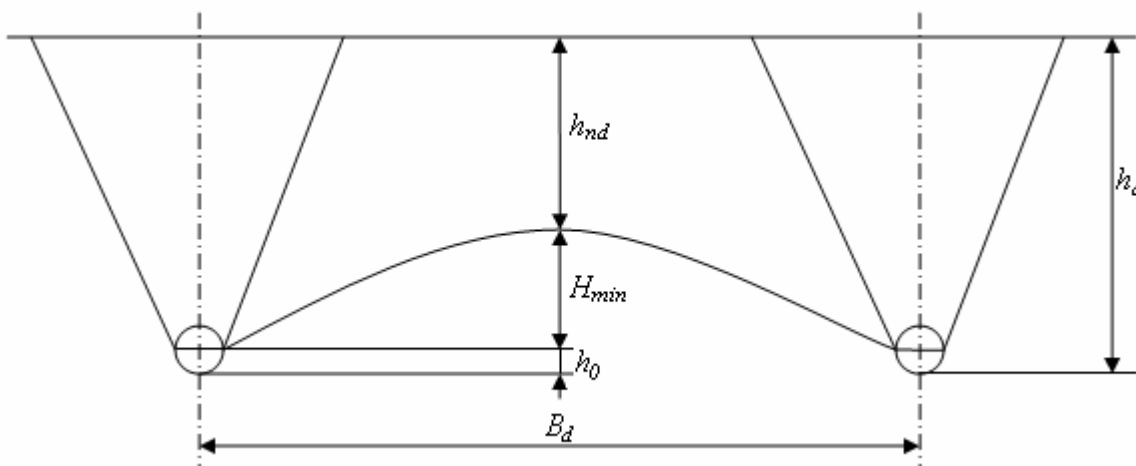
102-rasm. Yotiq zovur chuqurligini aniqlash sxemasi
