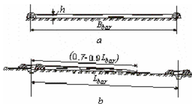
15-rasm. Yo‘laklab sug‘orish texnikasi hisobi uchun sxema:
