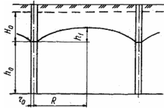
112-rasm. Hosil bo'lmagan suv ta'minoti uchun mukammal tik zovurning hisobiy sxemasi
