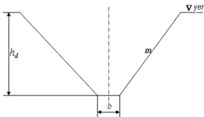
105-rasm. Ochiq yotiq zovurning ko‘rinishi
