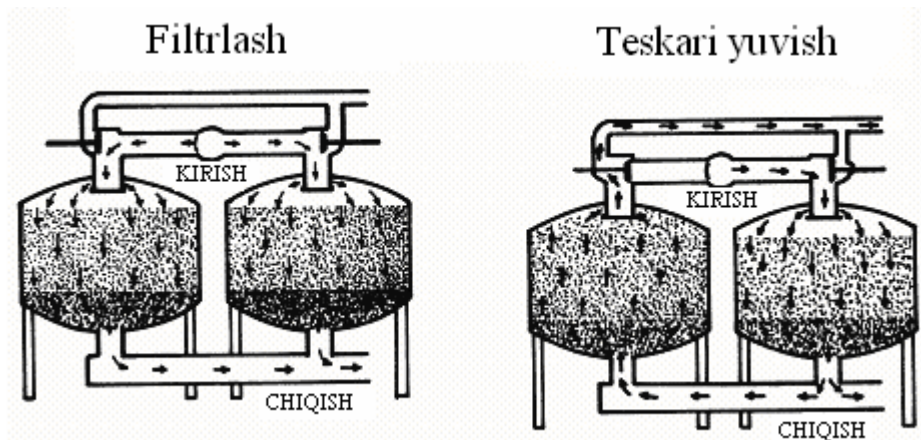
41-rasm. Qum-shag'al filtr
