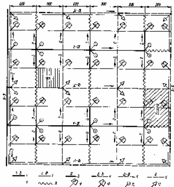
17-rasm. Kuban tipidagi sholi kartasi: 1, 2, 3-sug'orish tarmog'i; 4, 5, 6-tashlama; 7-yo'l; 8-marza; 9, 10, 11-suv berish inshooti; 12-suv tashlash inshooti
