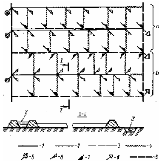
16-rasm. Krasnodar tipidagi sholi kartasi ( a -bir tomonlama, b -ikki tomonlama suv berish): 1-shohariq; 2, 3-tashlama; 4-marza; 5, 6-suv berish inshooti; 7, 8-suv tashlash inshooti; 9-kollektor
