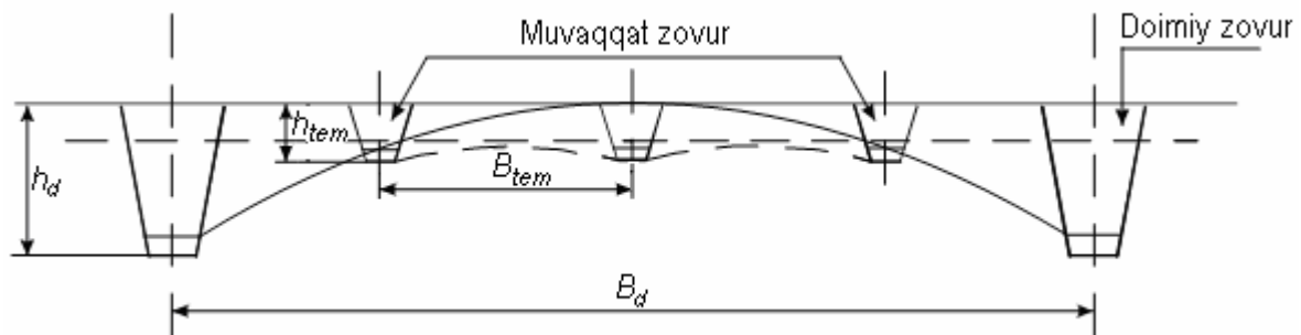
100-rasm. Muvaqqat zovurlar
