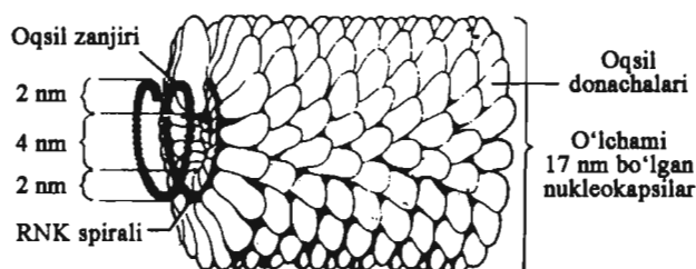
17-rasm. Tayoqchasimon tamaki mozaikasi virusining tuzilishi.
