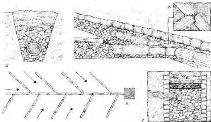
2.5-rasm. Bog'-parklarda drenaj tizimini qurish.
