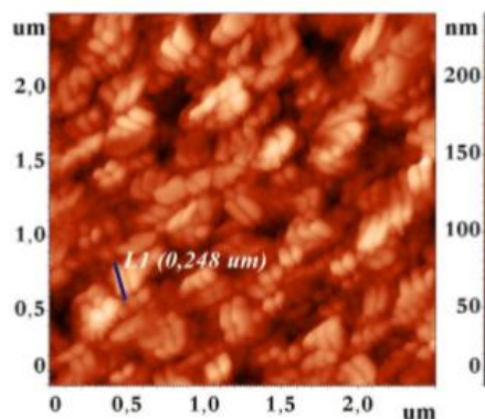
4-rasm. PbSe plyonkasining AFM tasviri, skanerlangan maydonning o'lchami 3 mkm x 3 mkm.
