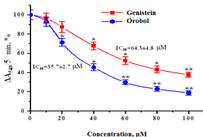
Figure 2. Effect of genistein and orobol isoflavones on \text{Fe}^{2+} -ascorbate-induced LPO in turtle liver mitochondria (* P<0,05 ; ** P<0,01 ; n=6 ).
