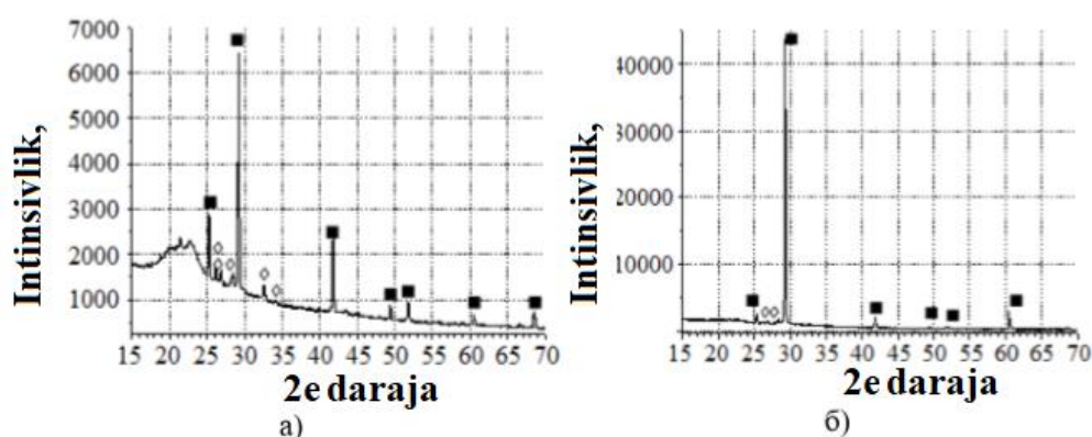
1-rasm. PbSe (a) va Al-PbSe (b) plyonkalarining diffraksiya naqshlari.
